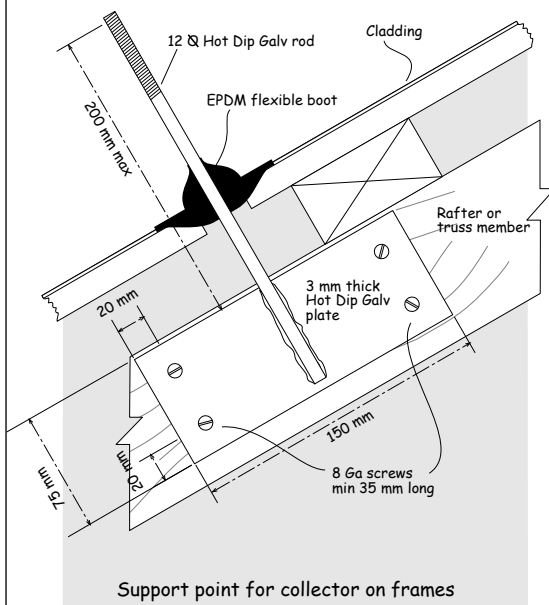
Figure 16: Stud fixing Paragraph 6.4.1 c)
